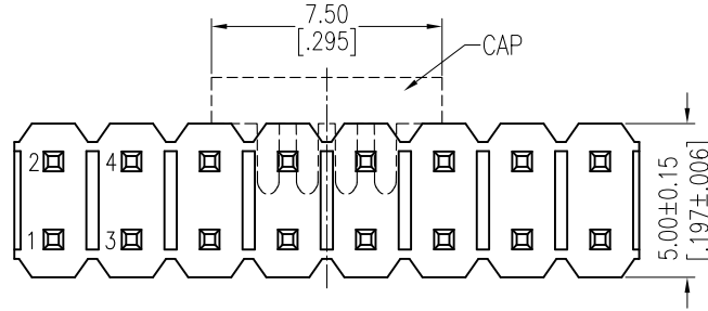
Dual Numbers
