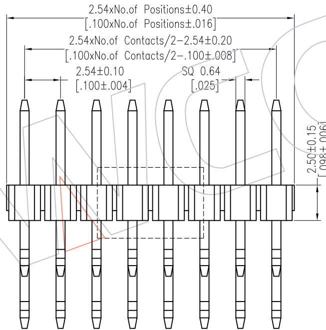
Dual Numbers
