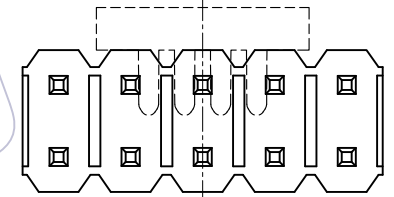
Odd Number
